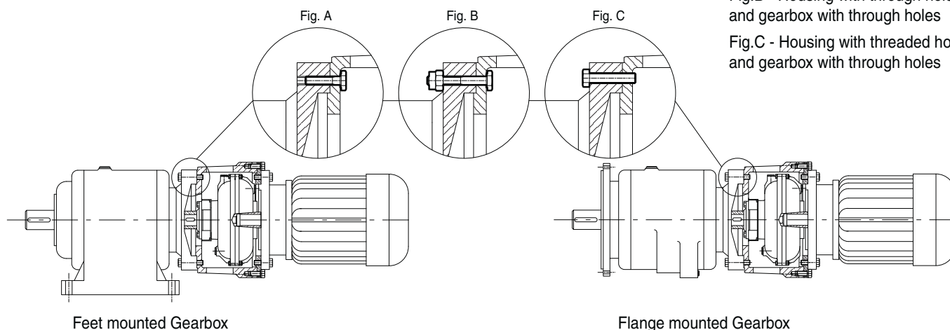
Feet mounted Gearbox
