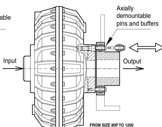
ROTOPIN flexible coupling
