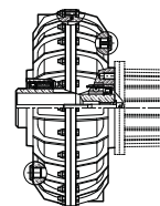
ROTOFUID DCF COUPLING
