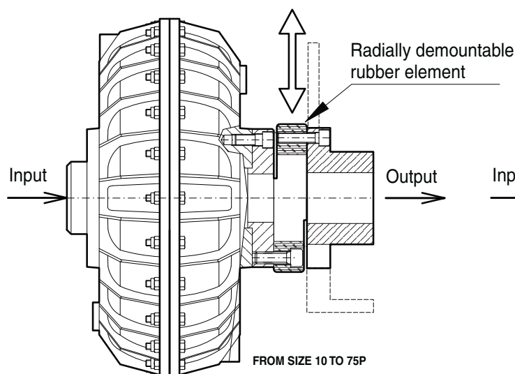
ROTOFLEXI flexible coupling
