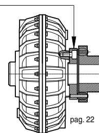
ROTOFLUID ALFA K-AB with ROTOPIN flexible coupling
