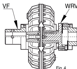
ROTOFLUID ALFA K-VF for "reverse mounting"
