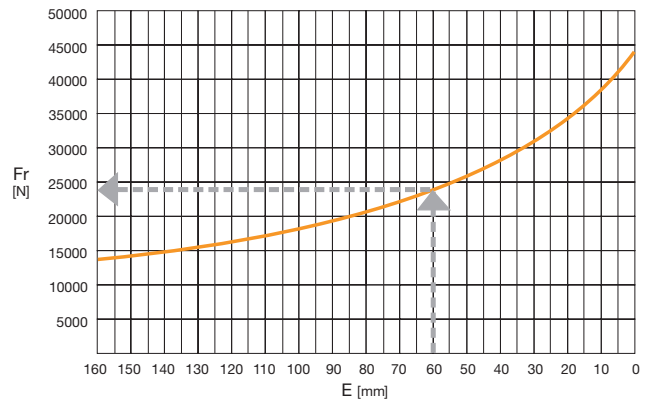
Example of bearing life chart for input and/or output shaft versions
